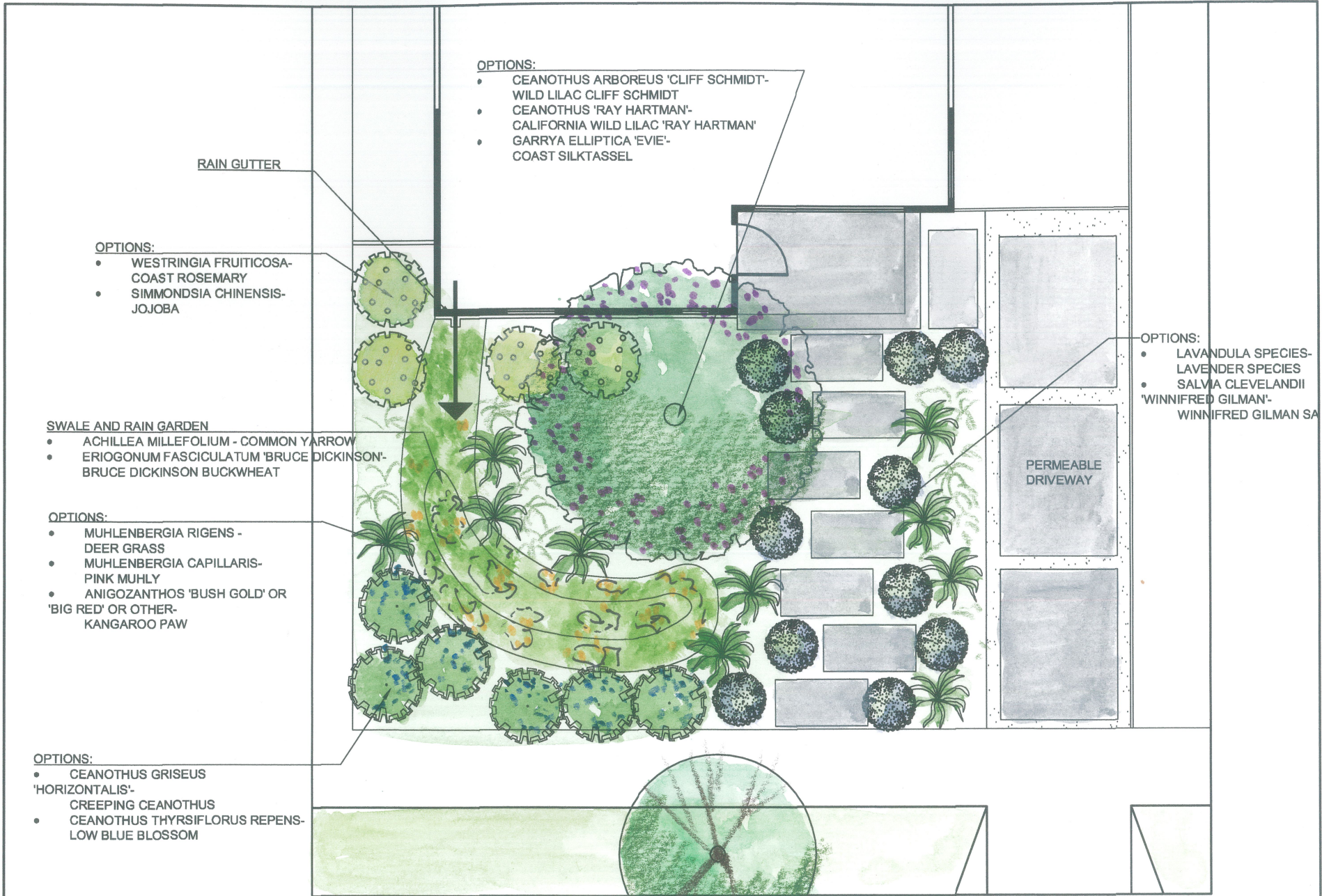
PLAN VIEW FRONT YARD RAIN GARDEN SUNNY EXPOSURE
